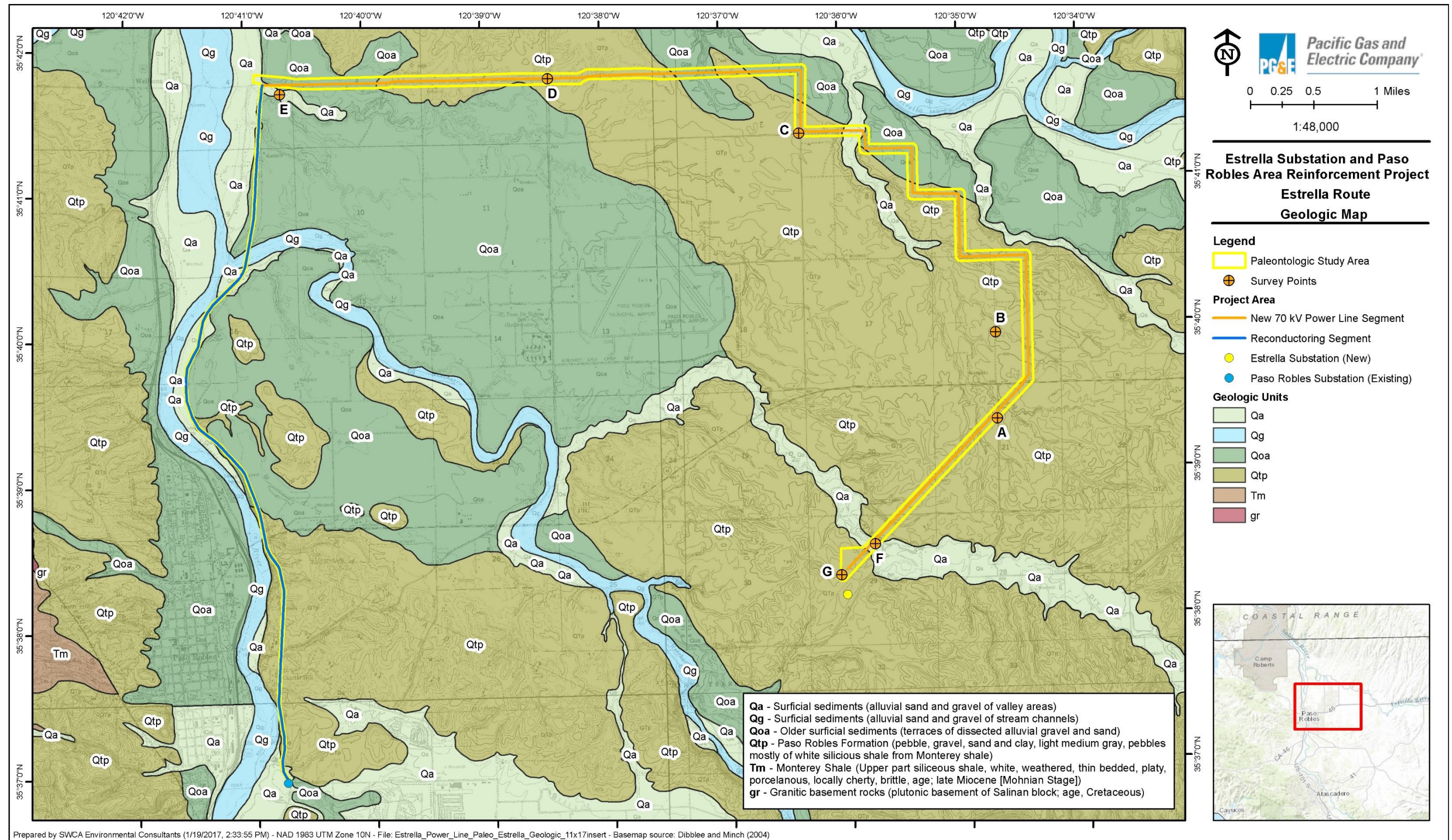
Figure 3. Geologic Map of the Estrella Route
