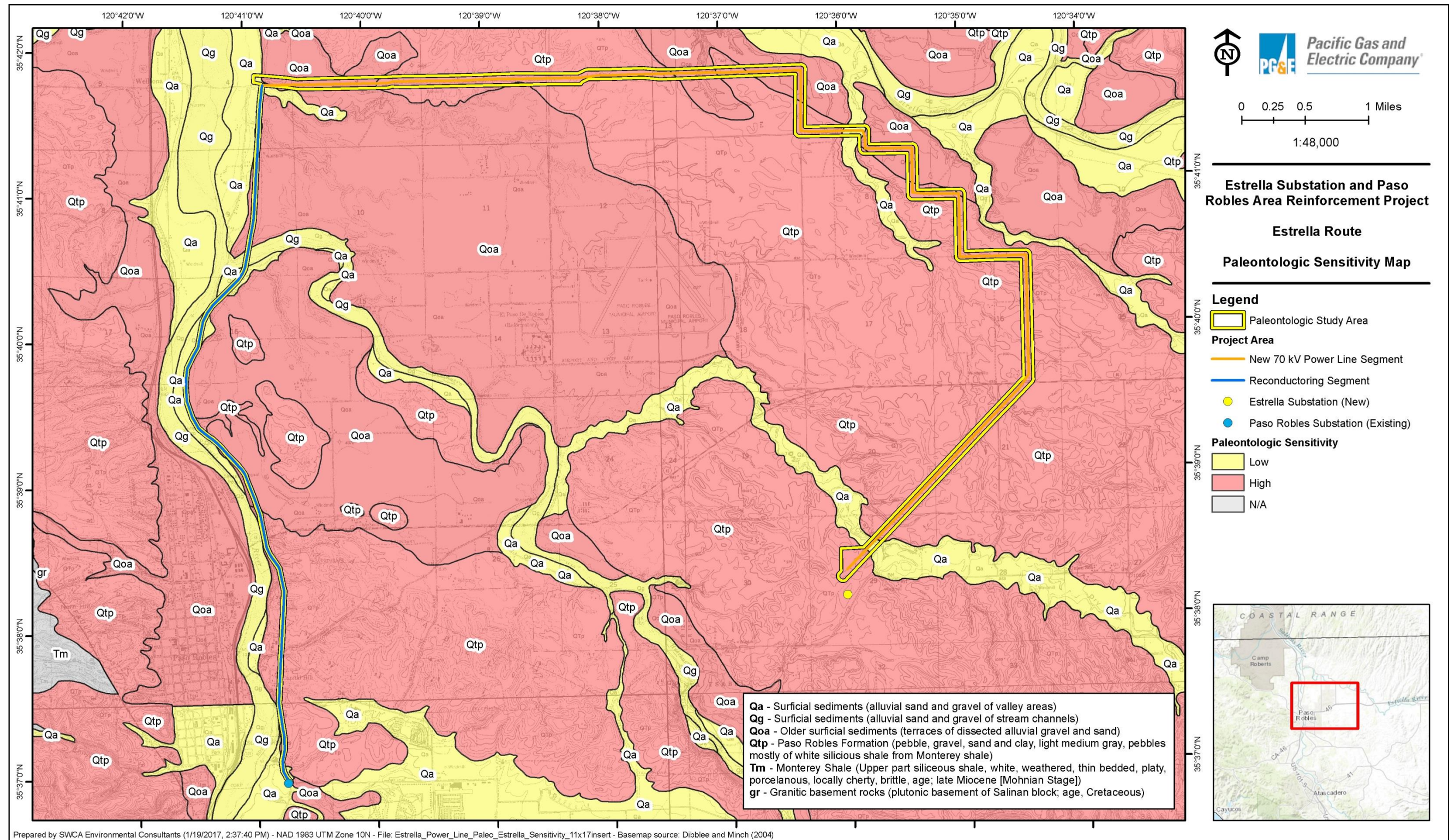
Figure 4. Paleontological Sensitivity for the Estrella Route
